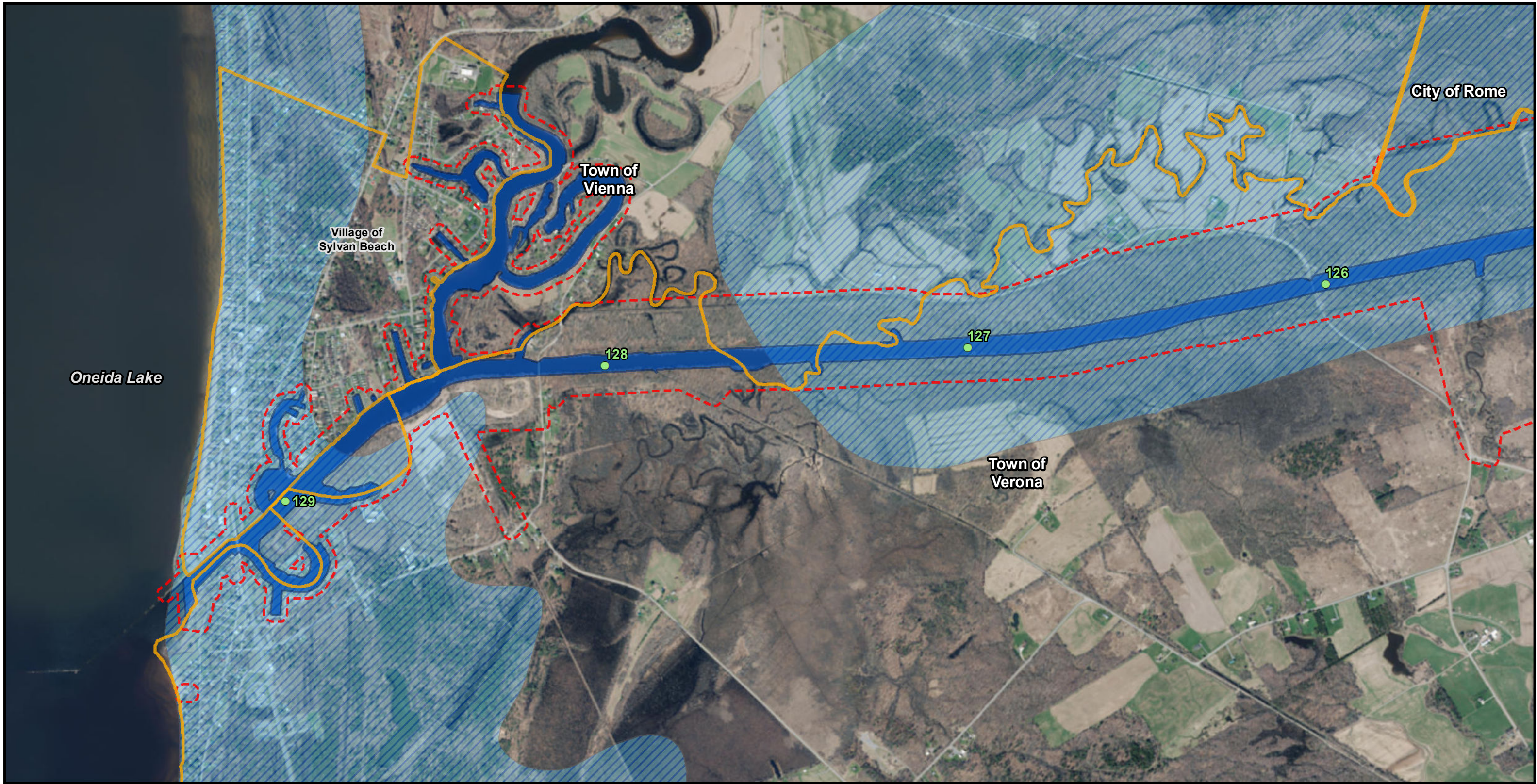
Figure 58F: Aquifers
